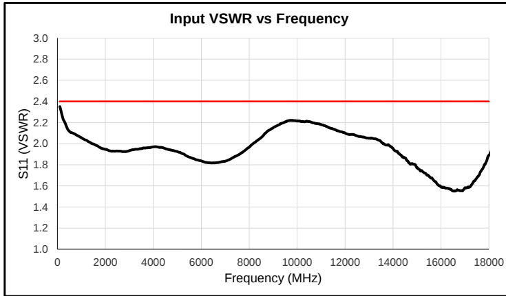
Typical Performance @ 23°C (Reference S/N 2162302)
