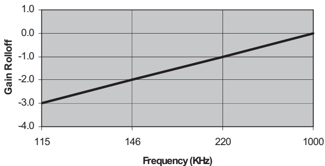
Low Frequency Gain Rolloff (dB)
