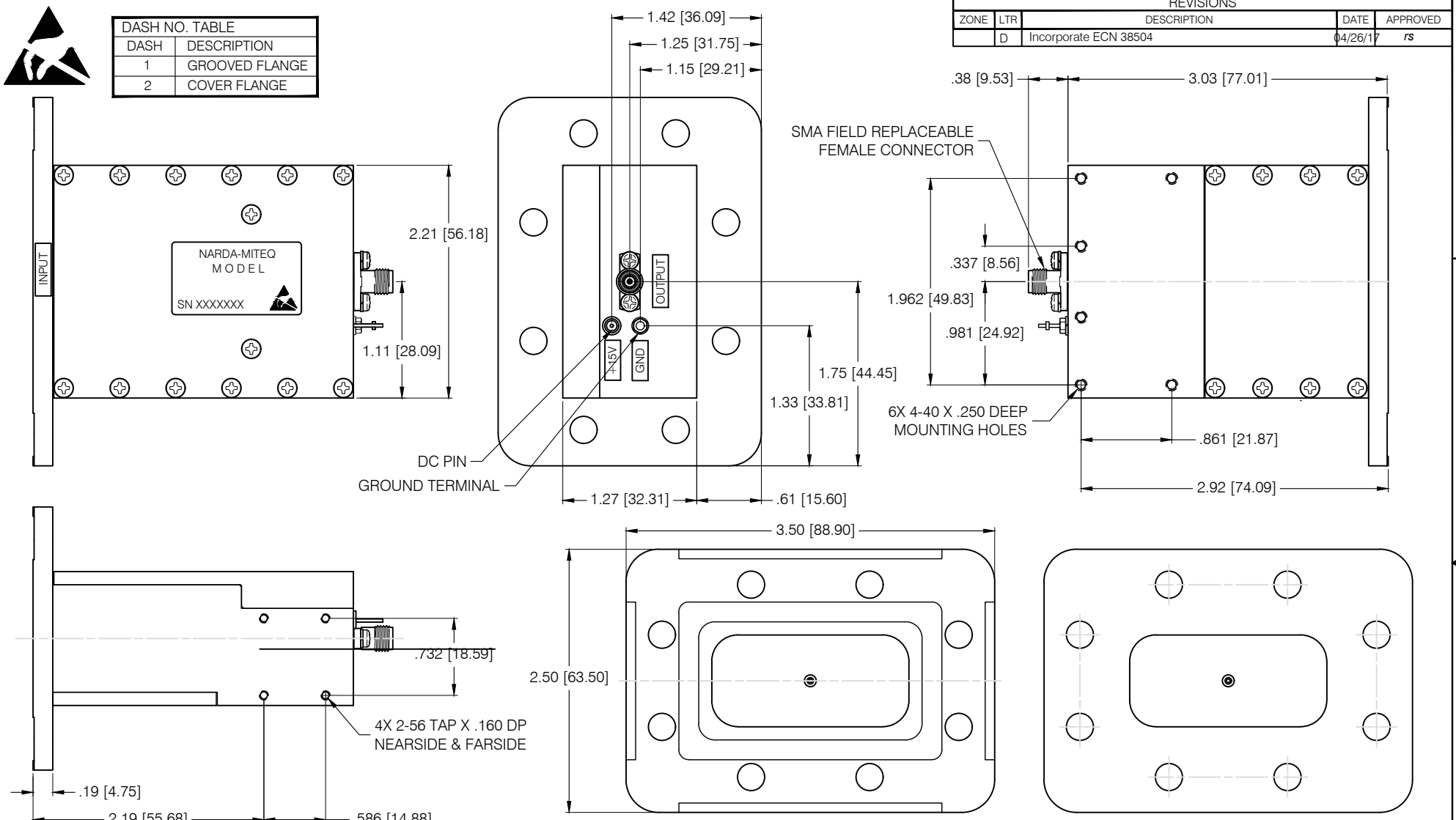
DASH 1 - GROOVED FLANGE CONFORMS TO UG1353/U WR187 FLANGE DASH 2 - COVER FLANGE CONFORMS TO UG1729/U WR187 FLANGE
